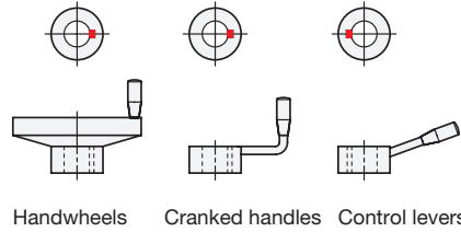
Positioning of the keyway:
